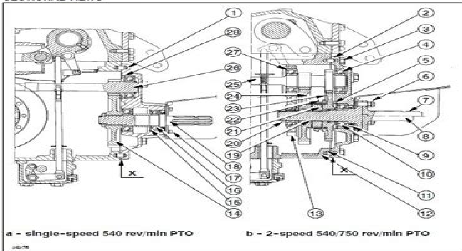
Cross-sectional views of single- and 2-speed PTO
