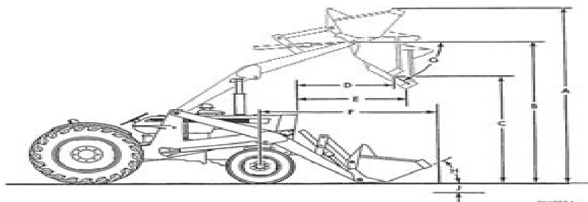
Figure 1 - Loader Specifications
