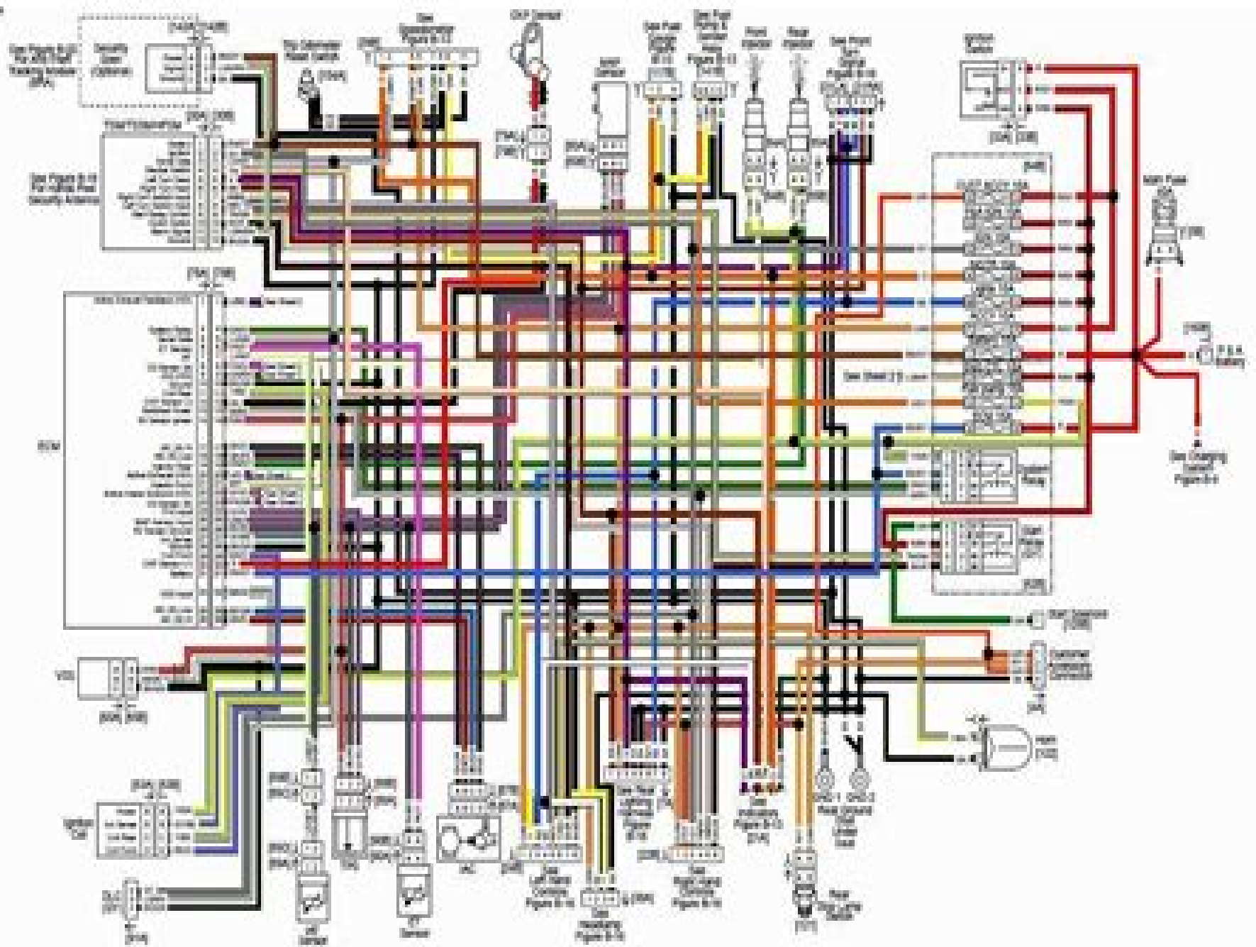
Figure B-11. Main Harness (1 of 2): 2010 Toyota (PHEV, FHEV, and FCEV)
