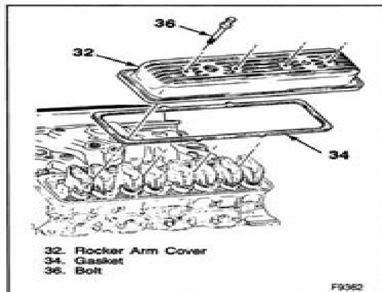
Figure 18—Rocker Arm Cover (5.0L and 5.7L Engines)
