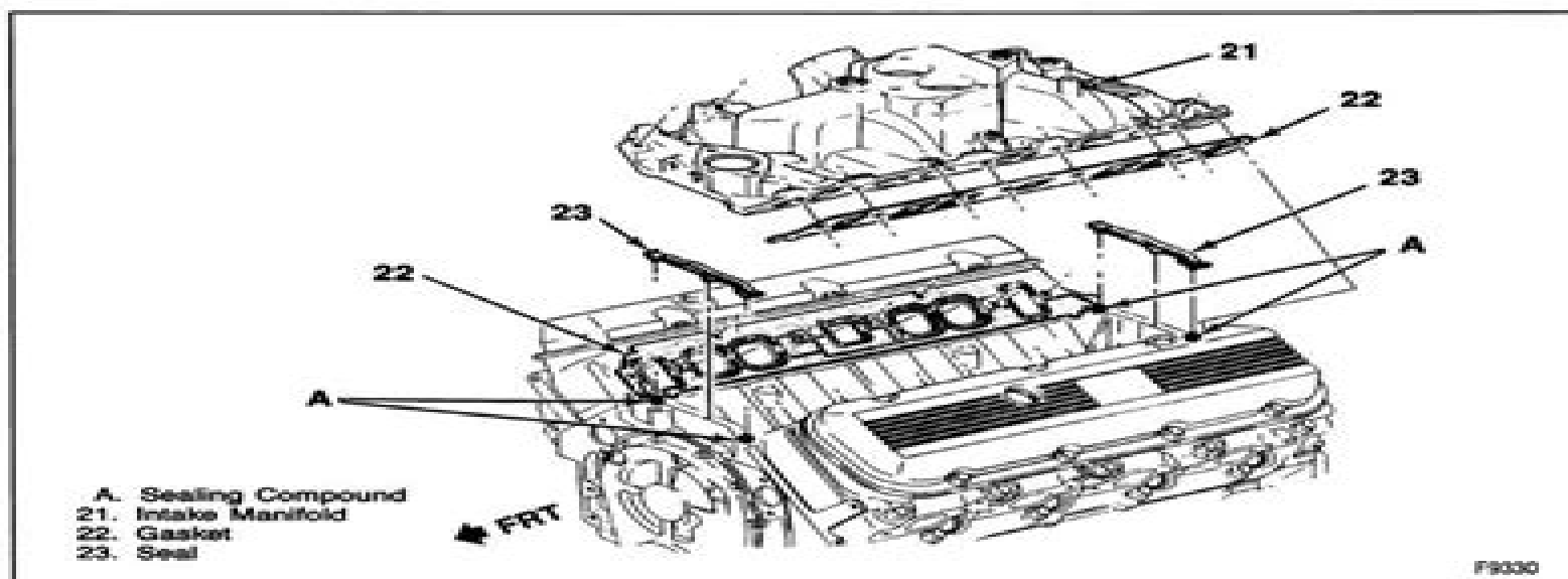
Figure 17—Intake Manifold (7.4L Engines)
