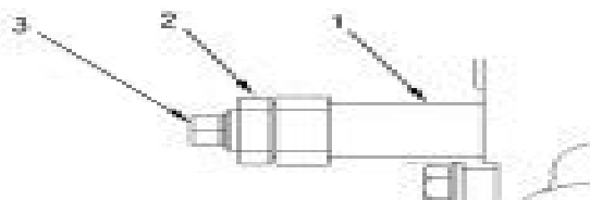
Illustration 78 g00627562 Hold relief valve (1) and loosen locknut (2). Slowly turn hex cap (3) counterclockwise until the equipment is lowered to the ground.
