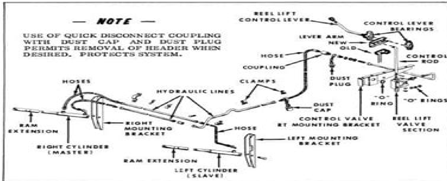
Figure AA-9. Details of Reel Lift Hydraulic Lines, Cylinder, Control Valve and Lever.
