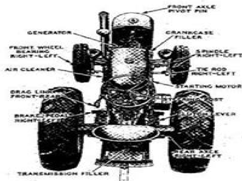
Figure 4. Lubrication—Models S and SO
