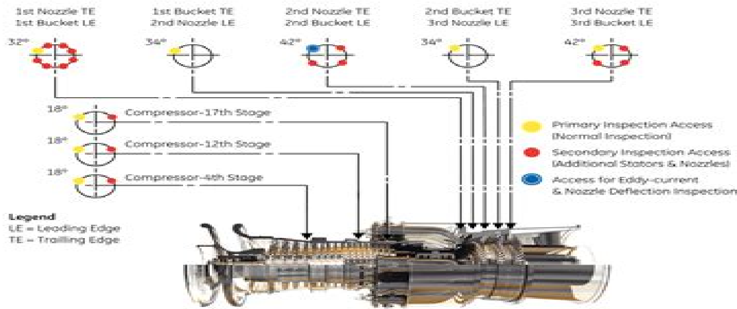
Figure 3. GE03 gas turbine borescope inspection access locations
