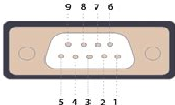
RS232 DB-9 Male Pinout
