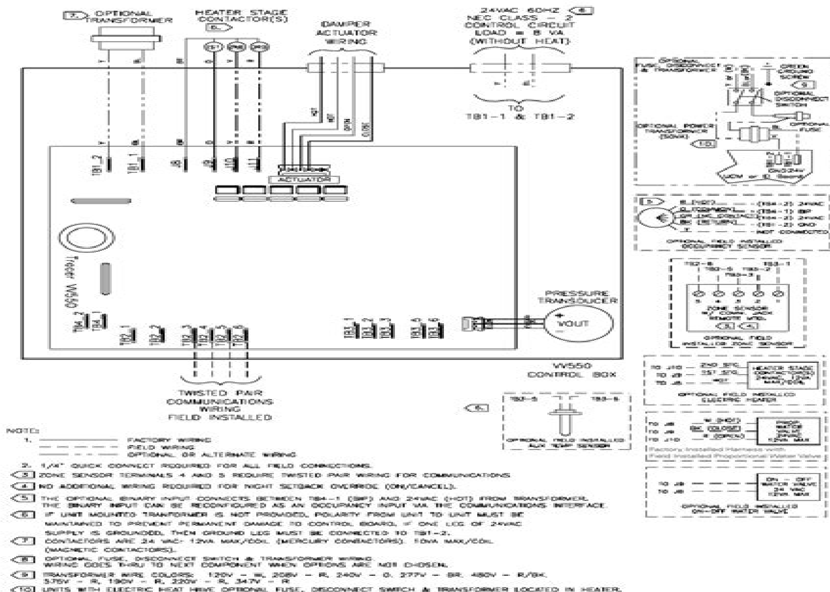
Figure 46. VV550 single duct control diagram
