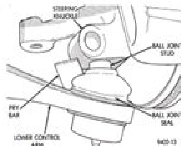
Fig. 24 Separate Ball Joint Stud from Knuckle Assembly
