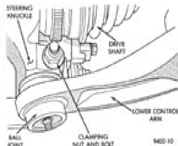
Fig. 23 Steering Knuckle To Ball Joint Clamp Bolt
