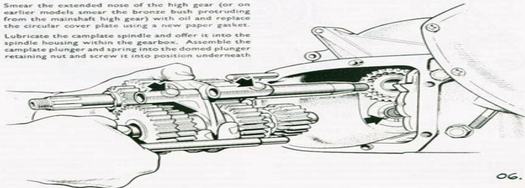
Fig. D11. Reassembling the gearbox components. Arrows indicate camplate rollers in position and thrust washer correctly located
