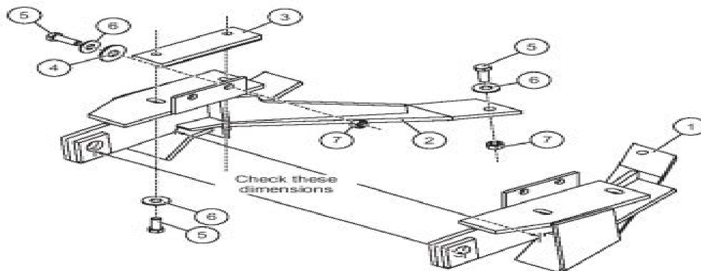
7125 Mount Kit
