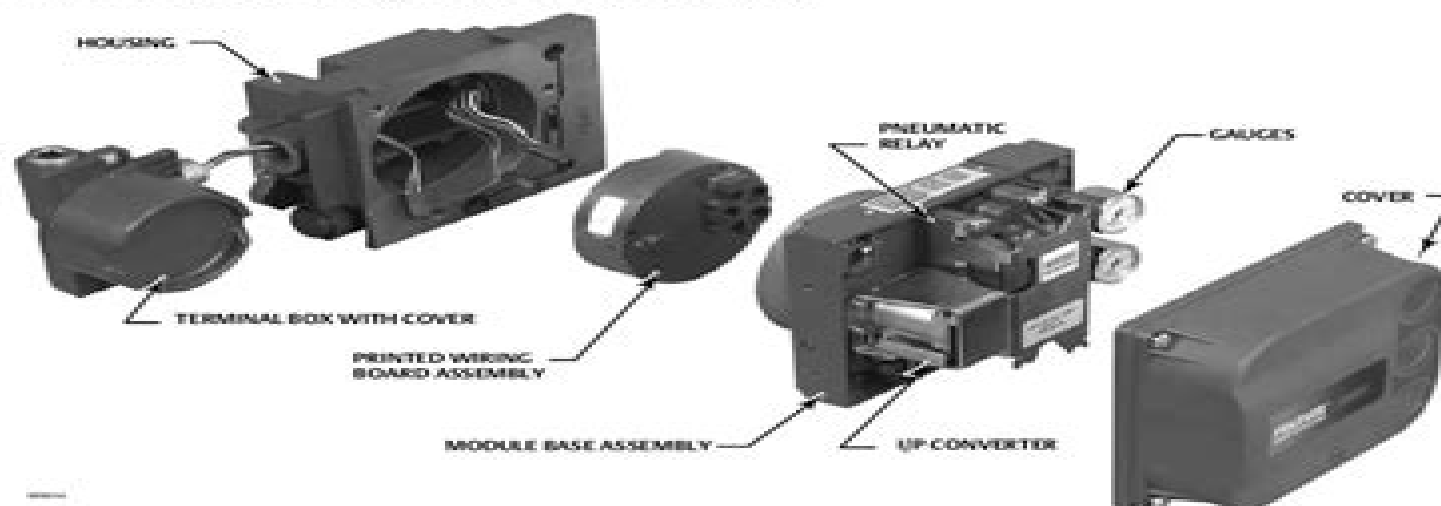
Figure A-4. FIELDVUE DVC6200 Digital Valve Controller Assembly
