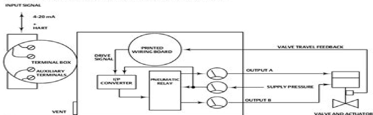
Figure A-3. FIELDVUE DVC6200 Digital Valve Controller Block Diagram
