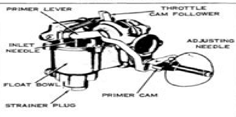
Figure 4-3. Carburetor for 3 H.P. Motors
