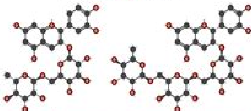
Cyanidin-3-O-rutinoside
