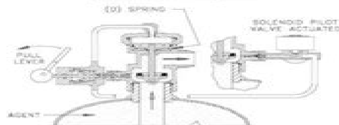
Cylinder Valve - Actuated Mode
