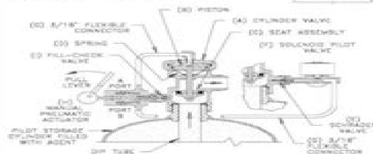
Cylinder Valve - Standby Mode
