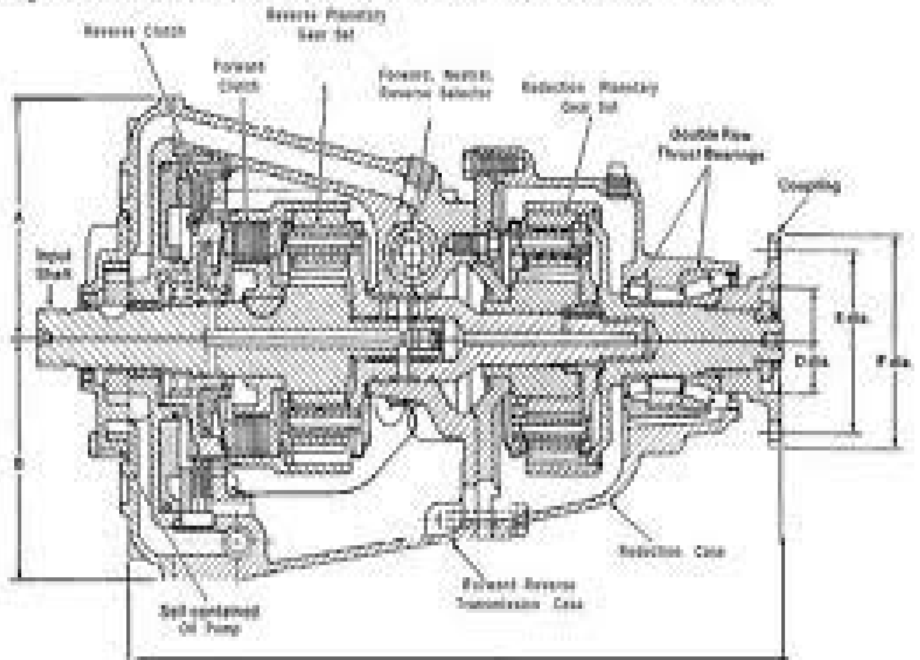
Figure 3 Installation drawing for In-Line transmissions (2.10:1.0) ratio illustrated
