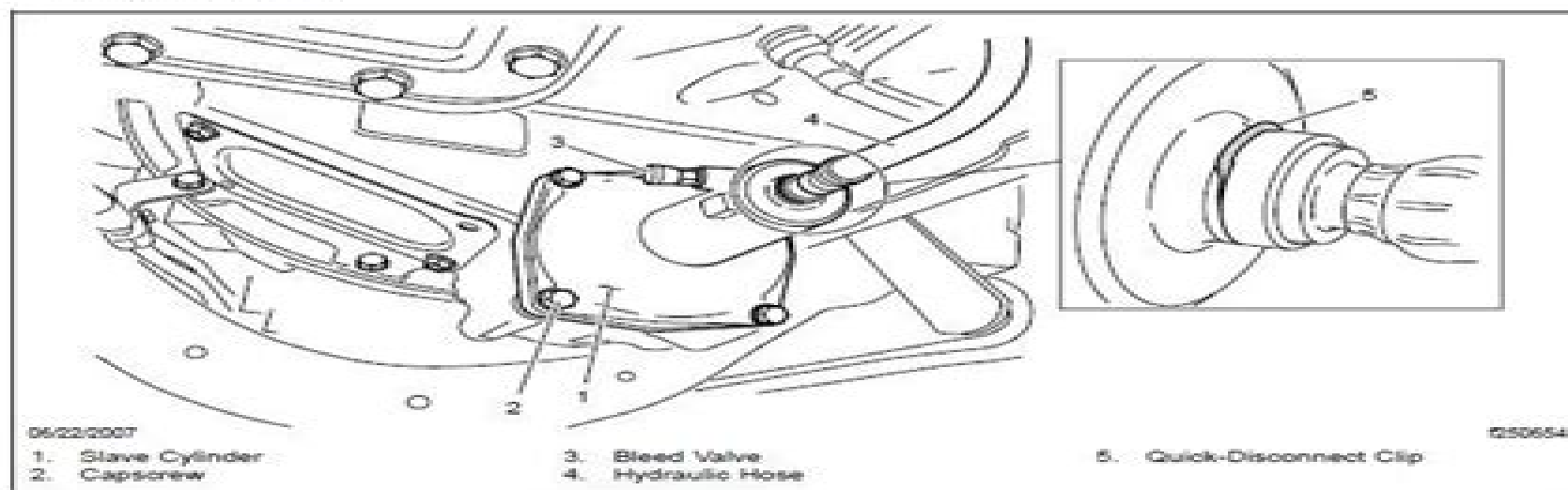
Fig. 1, Clutch Slave Cylinder
