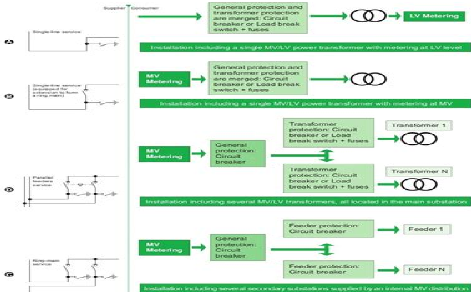
Fig. B8: A: Single line service. B: Single line service with provision for extension to ring main or parallel feeder service. C: Ring main service. D: parallel feeder service
