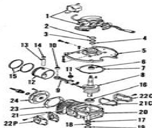
Fig. E2-21 - Exploded view typical of AV750 models. Some models may have breaker point type magnets.
