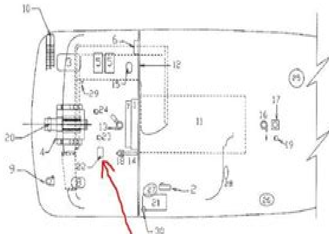
SIGNATURE 260 ENGINE COMPARTMENT LAYOUT
