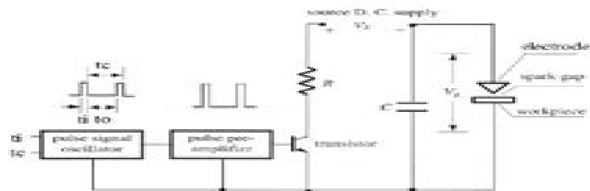
Figure 3. Transistorized RC power circuit
