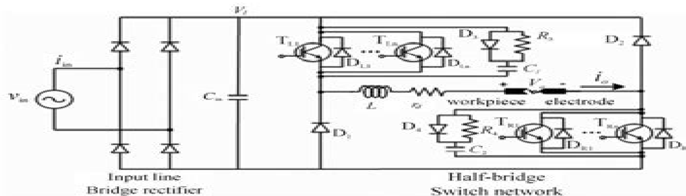
Figure 5. Circuit diagram of the HSEDMD power generator using a half-bridge network
