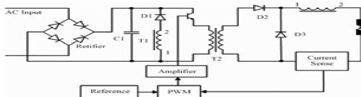
Figure 4. Energy-saving EDM power supply developed by Harbin Institute of Technology
