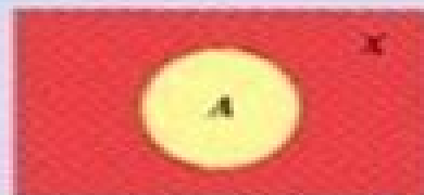
A^c is shaded
