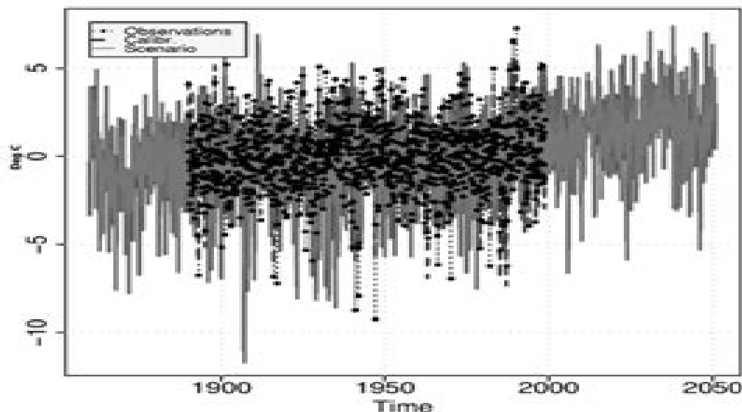
Fig. 1. Example of downscaled monthly 1890–1998 January mean temperature for Oslo-Bjørnsnes derived with clim.pact . The example is based on the ECHAM4/IPPC3 model and the IPCC IS92a-based GSDMO integration. (The GSDMO scenario includes the effects of greenhouse gases, tropospheric ozone, and direct plus indirect effects of industrial aerosols). The predictor used for calibration was gridded temperature described by Bengtsson [2001].
