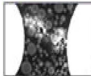
Underfill Cracking
