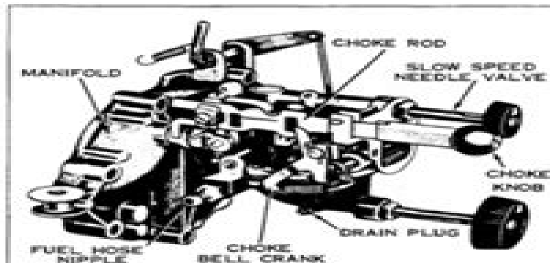
Figure 4-2. Carburetor for Late 12 H.P. Motors
