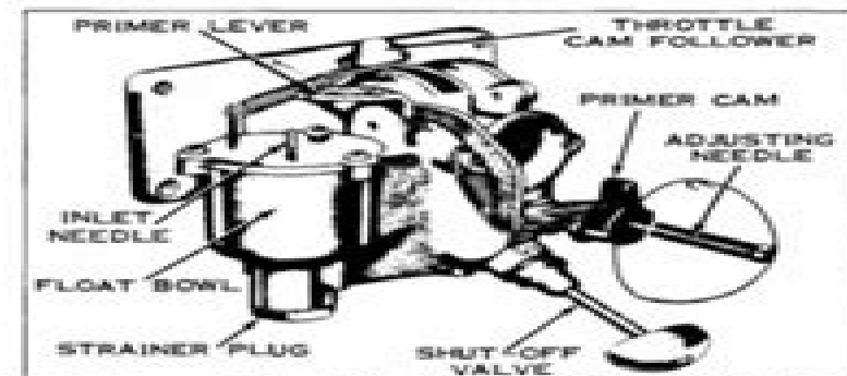
Figure 4-1. Carburetor for SD10, SD11 and 5 Standard Motors
