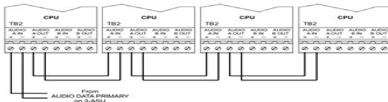
Figure 1-2: Class B network audio riser wiring
