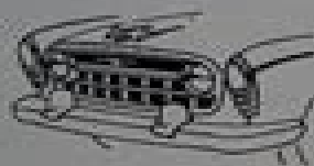
1957 Series 10 Rambler
