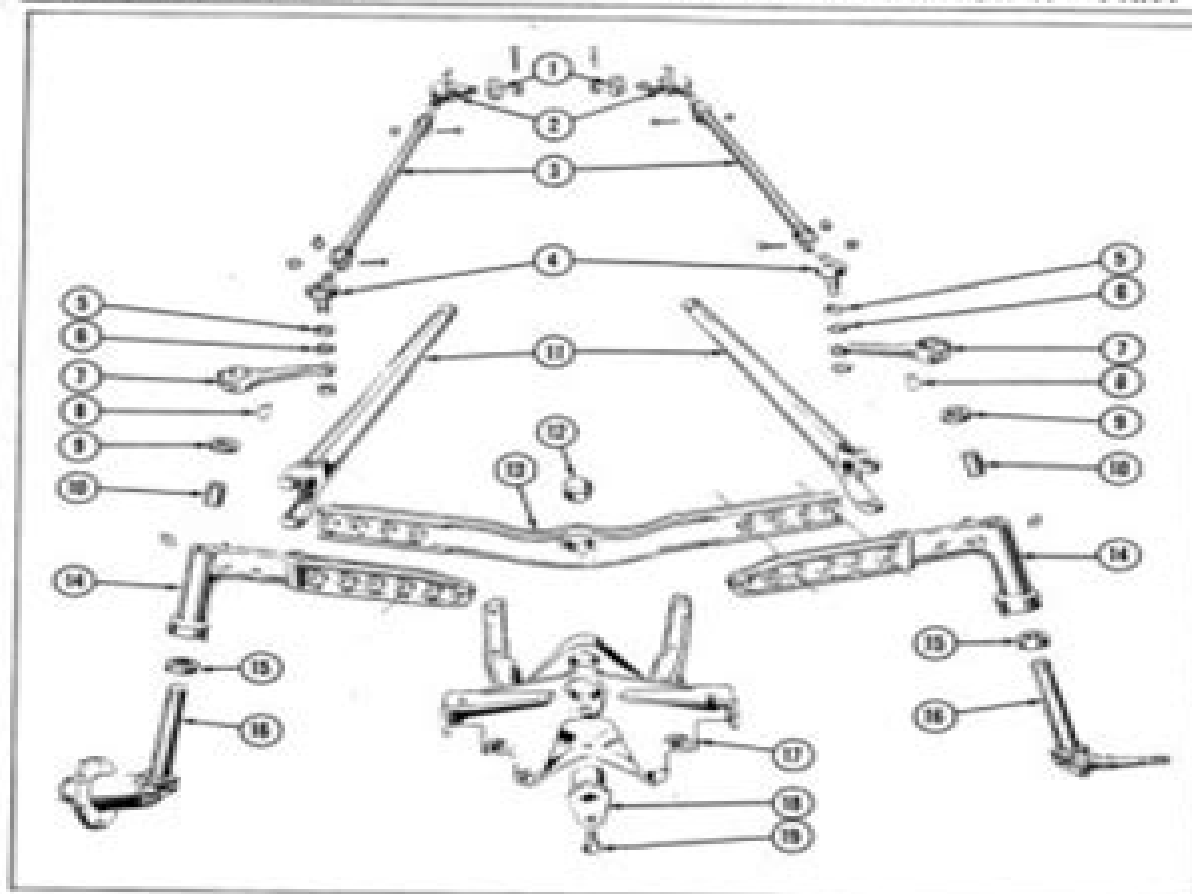
Fig. 1 - MF and TD 35 Front Axle Assembly Nomenclature
