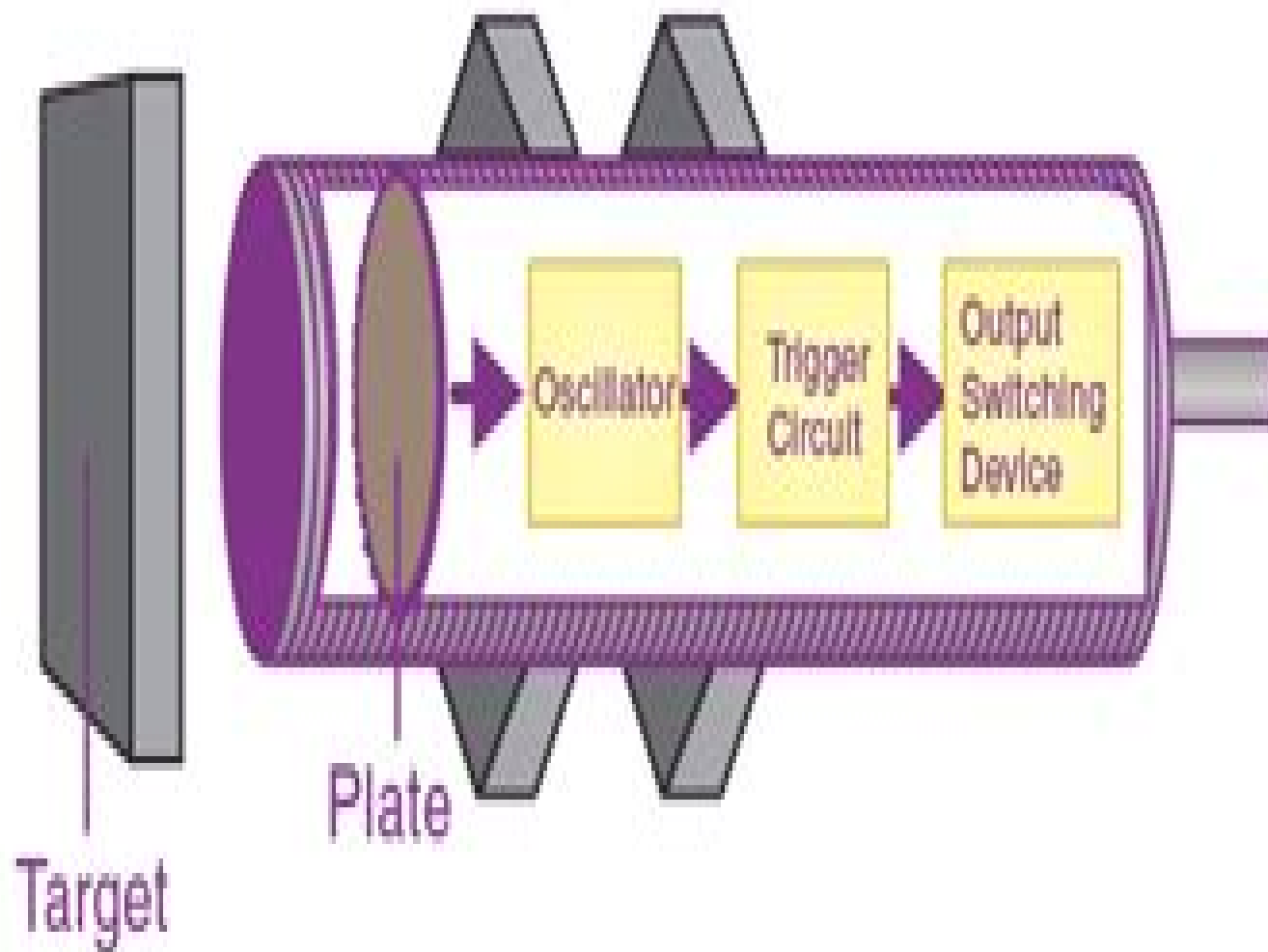
Capacitive Sensor
