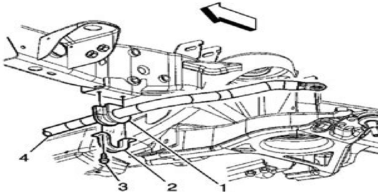
Fig. 3: Stabilizer Shaft, Bracket, Bolts & Insulators Courtesy of GENERAL MOTORS CORP.
