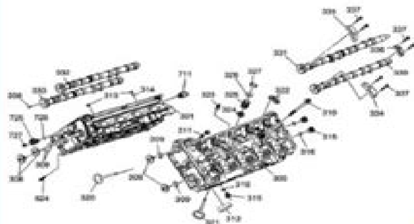
Fig. 27: Cylinder Head Assemblies Courtesy of GENERAL MOTORS CORP.
