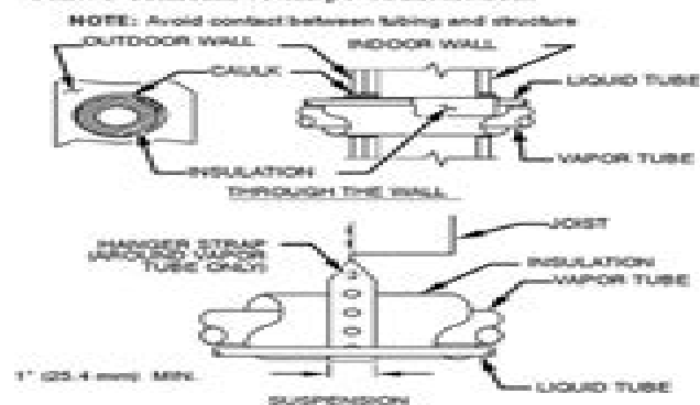
Fig. 1 - Piping Installation
