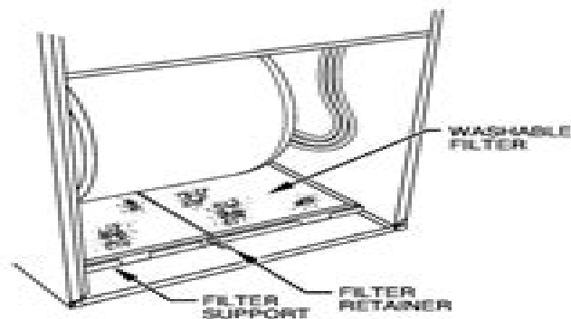
Fig. 3—Bottom Filter Arrangement
