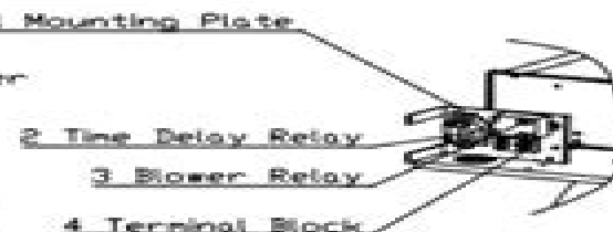
Fig. 22 – FFMA and FMA4 (Sizes 30 &amp; 36) Expanded View - Duct Components, Blower &amp; Electrical Parts
