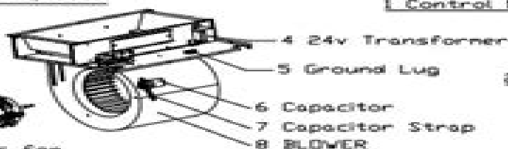
Fig. 22 – FFMA and FMA4 (Sizes 30 &amp; 36) Expanded View - Duct Components, Blower &amp; Electrical Parts
