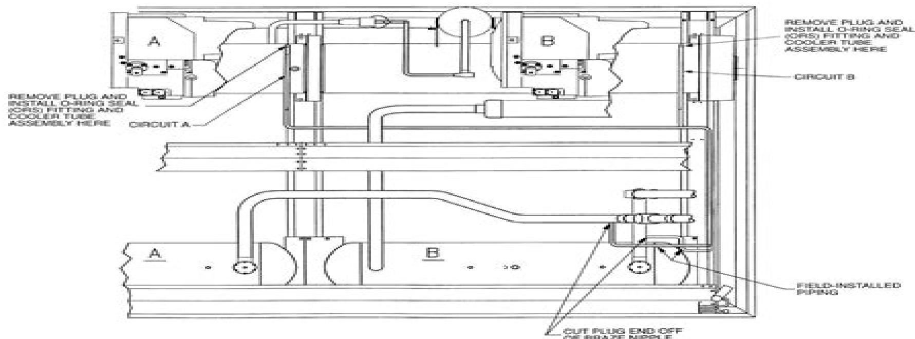
Fig. 1 — Installing Fittings, 30GXN,R (Typical Size 080-150, 160 Shown)
