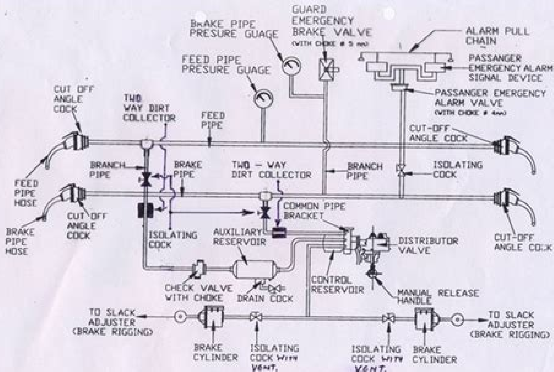
TWIN PIPE GRADUATED RELEASE AIR BRAKE SYSTEM
