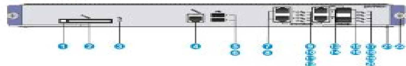
Figure 1 Front panel
