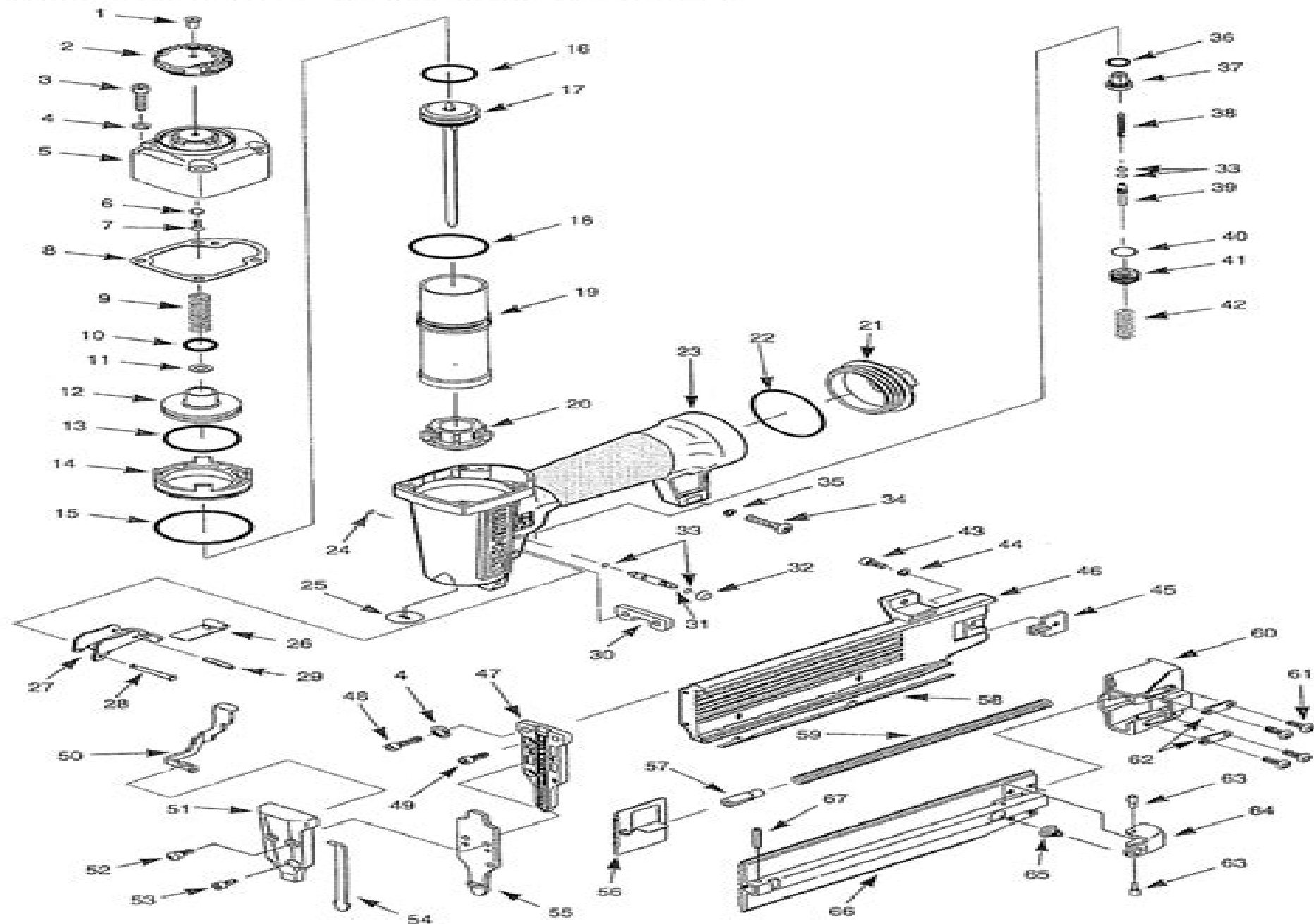
Figure 5 - Replacement Parts Illustration For Nail
