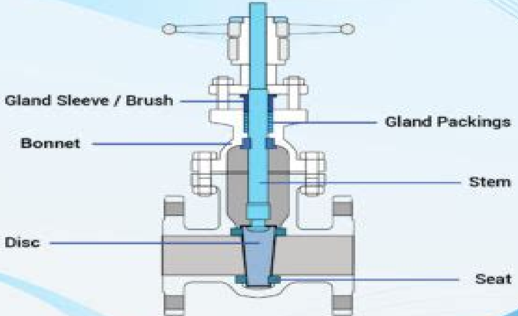
Valve Components
