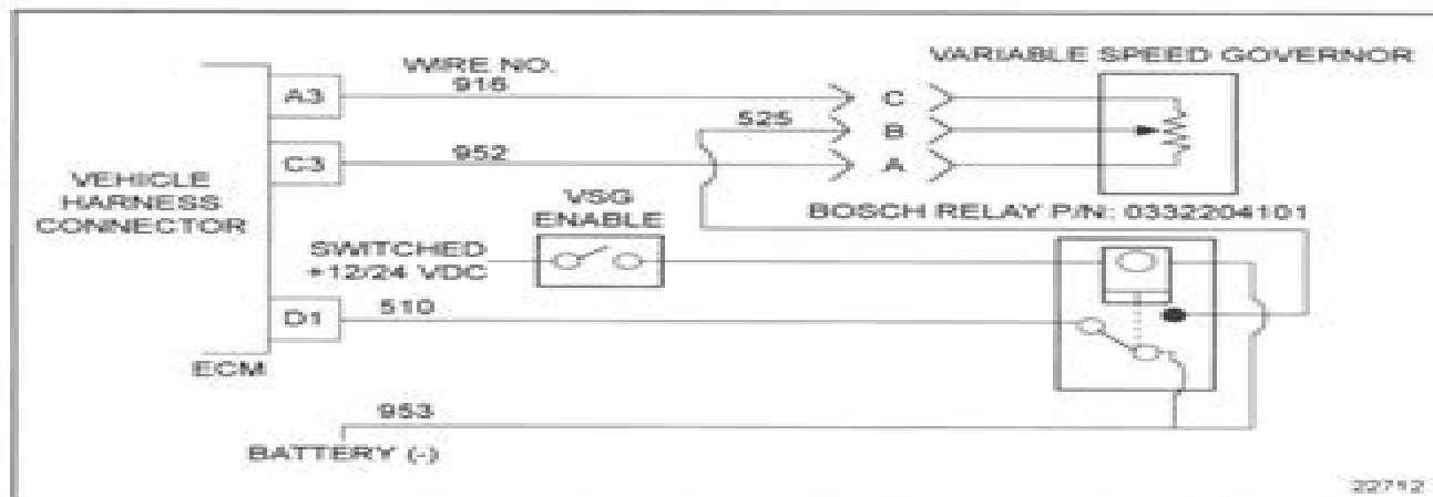
Figure 12-1 Variable Speed Governor Circuit
