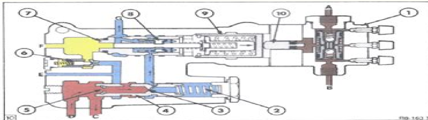
Trailer Brake Valve - Brakes Applied With Maximum Brake Pedal Pressure
