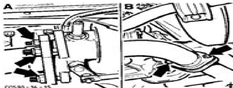
Fig.4. Fixture of front exhaust pipe. A - To turbocharger B - To catalytic converter
