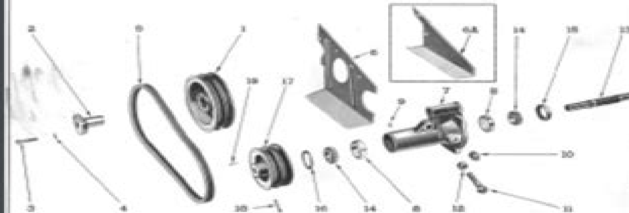
Figure 20 - Drive Pulley and Driven Pulley Housing Assemblies
