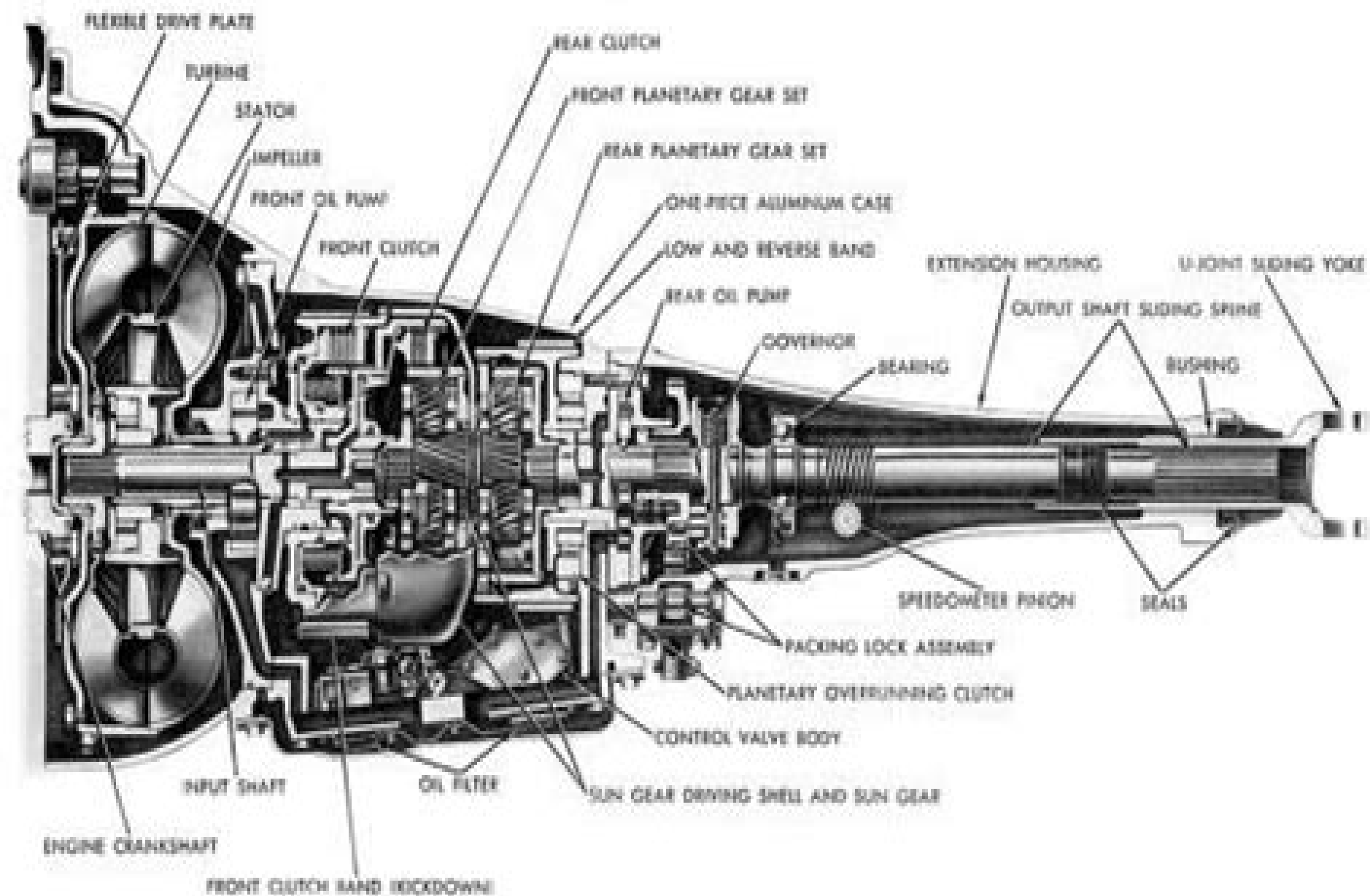
Torqueflite Transmission and Torque Converter (A-727-A and B)
