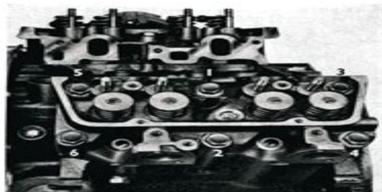
Fig. 8 Cylinder Head Bolt Tightening Sequence
