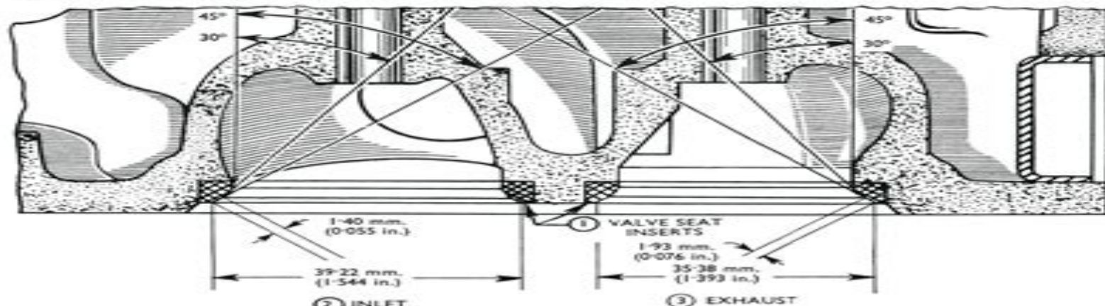
Fig. 9 Valve Seat Insert Machining Dimensions
