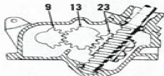
Fig. 3—Cross-sectional view of manual steering gear assembly showing correct installation of sector gears and wormshaft assembly. Refer to Fig. 2 for exploded view and parts identification.
