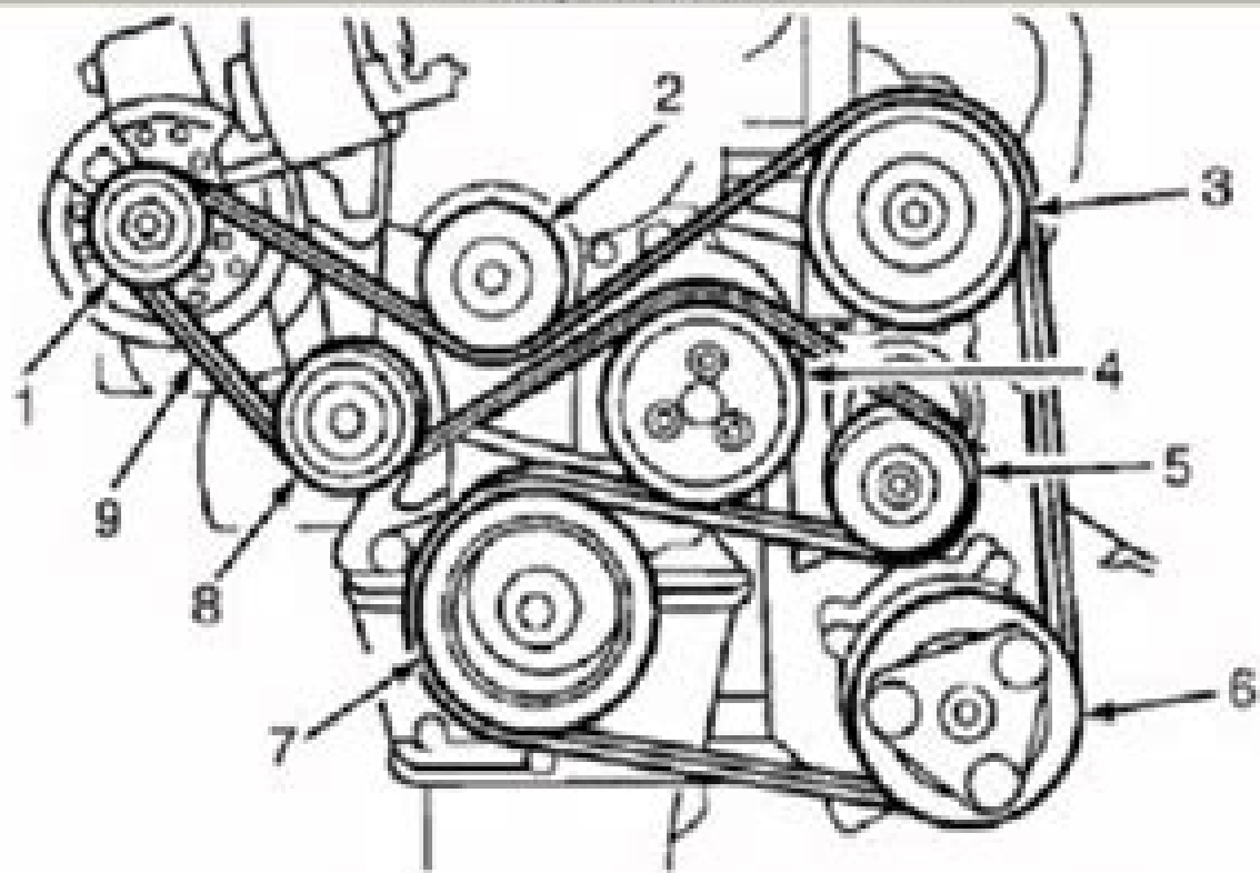
Fig. 9 Serpentine Belt Routing (Excerpt 2.28, VIN 3 - Excerpt 202) Courtesy of FORD MOTOR CO.
