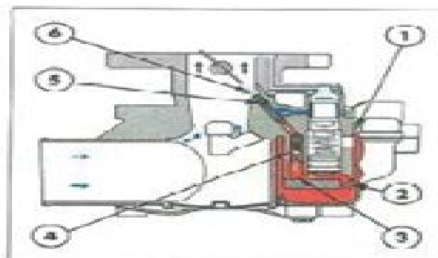
Figure 6 Accelerator Pump System
